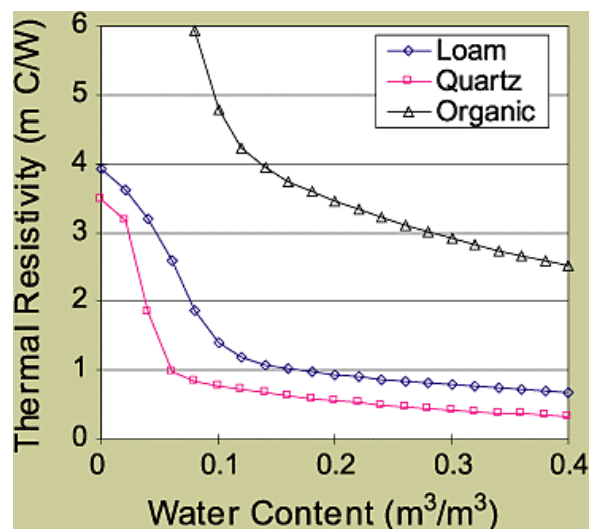
Fig. 2- Adding water to a porous material drastically decreases its thermal resistance.
